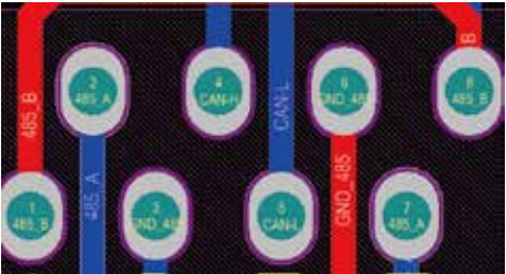
Port BMS 485/CAN
