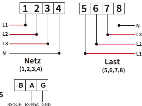
Abb. 7.18 EASTRON-Messer
